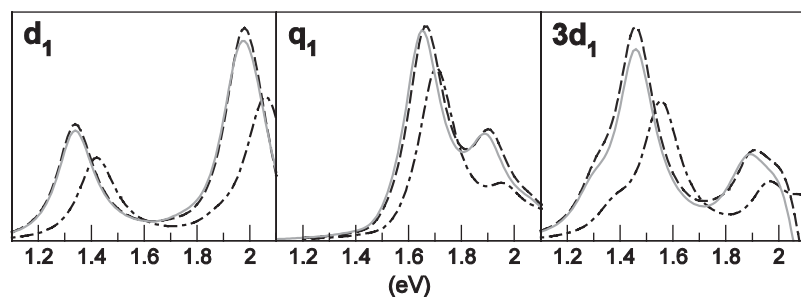
Figure 8. TPA cross sections (arbitrary units) of dipolar ( \mathbf{d}_1 ), quadrupolar ( \mathbf{q}_1 ) and 3-branched octupolar ( 3\mathbf{d}_1 ) chromophores obtained with different models for the second-order hyperpolarizability ( \chi^{(2)} ): vac-vac (dashed-dotted line), vac-tol (dashed line) and tol-tol (continuous line) (see main text).
