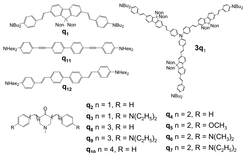
Figure 7. Molecular structure of quadrupolar compounds \mathbf{q}_1 – \mathbf{q}_{12} and branched chromophore 3\mathbf{q}_1 . Index n denotes the number of vinyl units (i.e., the number of double bonds in the conjugated bridge) for the arylidencyclohexanone chromophores \mathbf{q}_2 – \mathbf{q}_{10} .
