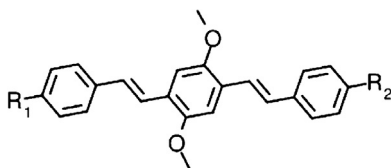
Figure 1. Structure of substituted PPV oligomer molecules. R_1 = H, NO_2, NH_2, CO_2H with R_2 = H and R_1 = NO_2, R_2 = NH_2 .
