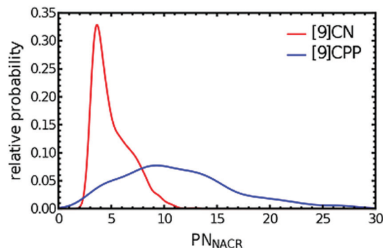
Fig. 7 Distribution of PN_{\text{NACR}} values, representing the number of ES-ENMs( S_1 ) that contribute to \text{NACR}_{12} at the moment of effective S_2 \rightarrow S_1 transition for NEXMD simulation of [9]CPP and [9]CN.
