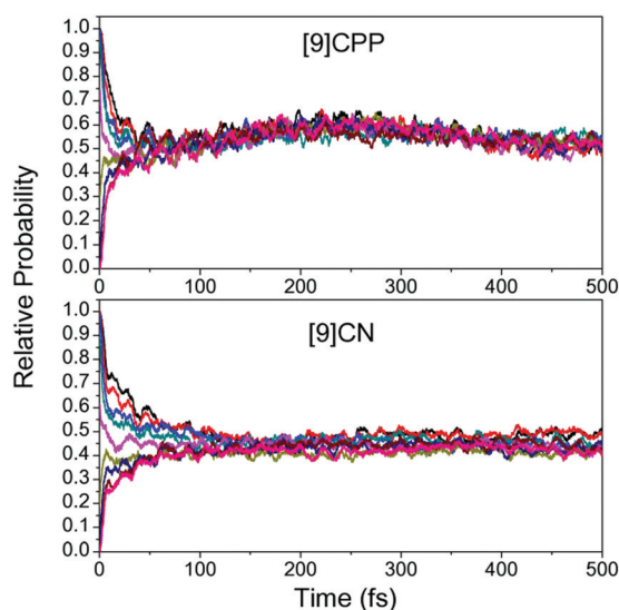
Fig. 6 Variation in time of the relative probability of each phenyl/naphthyl unit to retain a portion of the total electronic transition density during the NEXMD simulations of [9]CPP (upper panel) and [9]CN (lower panel) respectively.
