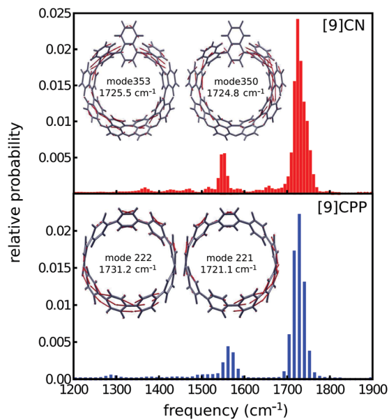
Fig. 8 Distribution of the projection of \text{NACR}_{12} at the moment of effective S_2 \rightarrow S_1 transition for each NEXMD simulation onto the basis of ES-ENM( S_1 ). Modes that represent the main contributions to \text{NACR}_{12} direction are shown.
