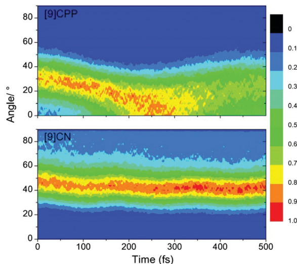
Fig. 5 Time evolution of the probability density of the dihedral angles between neighboring phenyl/naphthyl units during NEXMD simulations of [9]CPP (upper panel) and [9]CN (lower panel) respectively.
