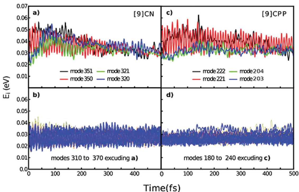
Fig. 9 Time evolution of the total energy of trajectories along (a) active normal modes, and (b) other normal modes excluding those plotted in part a for [9]CN, (c) active normal modes, and (d) all the normal modes excluding those plotted in part c for [9]CPP.
