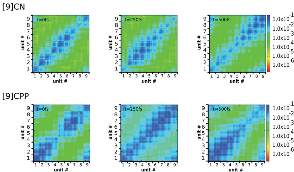
Fig. 4 Two-dimensional plots of transition density matrix elements for the current state, on the basis of chromophore unit atomic orbitals, at t = 0 fs, t = 250 fs and t = 500 fs for a representative NEXMD trajectory. The x and y axes denote spatial positioning of an electron and a hole in respective atomic orbitals for chromophore units ordered along the molecular backbone. The color coding is shown on the right hand side.
