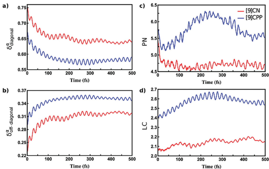
Fig. 3 The evolution in time of the diagonal \delta_{\text{diagonal}}^{\alpha} (a) and off-diagonal \delta_{\text{off-diagonal}}^{\alpha} (b) sums (eqn (3) and (4)) of the transition density matrix, phenyl/naphthyl-unit participation number \text{PN} (c), that measures the number of units over which the excitation is spread (eqn (5)), and \text{LC} (d), that measures the degree of separation between electrons and holes at different chromophores (eqn (6)).
