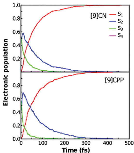
Fig. 2 Average population on each electronic surface as a function of time obtained from the time-dependent fraction of trajectories in each state during NEXMD simulations of [9]CN (upper panel) and [9]CPP (lower panel).
