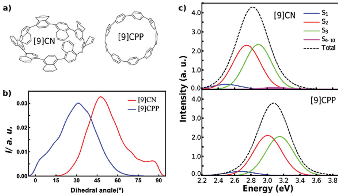
Fig. 1 (a) Schematic representation of [9]CN, and [9]CPP molecules; (b) dihedral angle distributions computed via ground-state dynamics simulations in thermal equilibrium at 300 K; (c) simulated absorption spectra of molecules along with separated contributions of different excited states.
