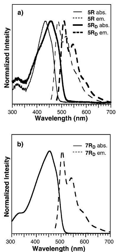
Figure 2. Absorption and emission spectra of (a) 5R , 5R D and (b) 7R D in toluene. The emission spectra were obtained by exciting at the corresponding absorption maxima.
