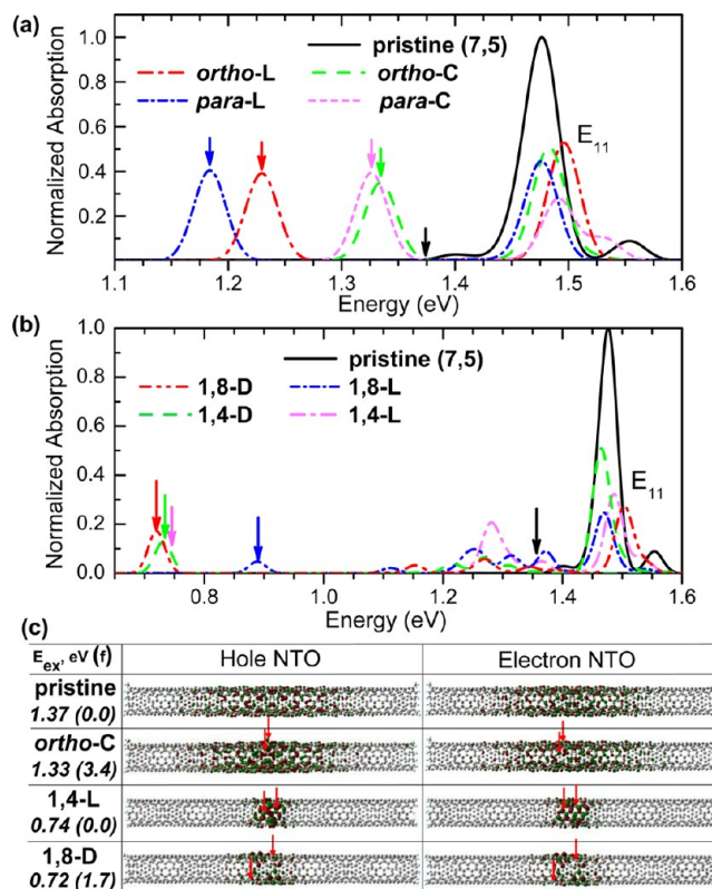
Figure 2. Comparison of calculated optical properties of hydrogenated and pristine (7,5) SWNT systems. (a) Absorption spectra for the ortho - and para - positions of hydrogen pair placed at circumferential (C) and longitudinal (L) orientations; (b) Absorption spectra with the 1,4- and 1,8- positions of hydrogen pair placed at diagonal (D) and longitudinal (L) orientations. Energy corresponding to the first excitation of each system is indicated by a vertical arrow. (c) Representative electron and hole NTOs corresponding to the lowest excited state of pristine and hydrogenated (7,5) SWNT systems. To the left of each NTO pair, the corresponding transition energy (eV) and oscillator strength (in parentheses) are given. The red arrows mark the position of adsorbed hydrogens.
